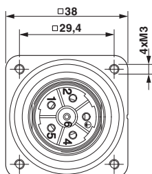
Dimensional drawing
